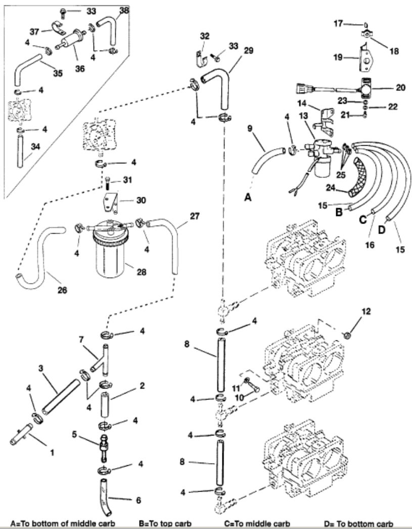
A=To bottom of middle carb B=To top carb C=To middle carb D= To bottom carb
